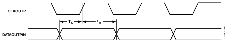
Figure 3. Output Timing
